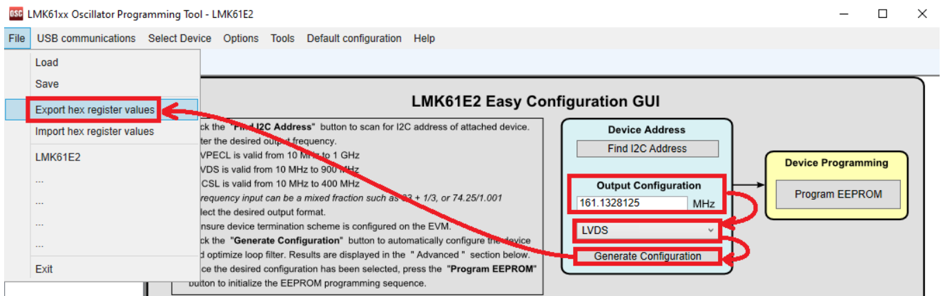
Figure 9 : LMK61xx Oscillator Programming Tool GUI
